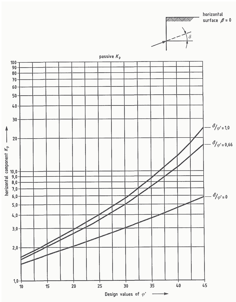
Figure C.2.1 — Coefficients K_p of passive earth pressure: with horizontal retained surface ( \beta = 0 )
