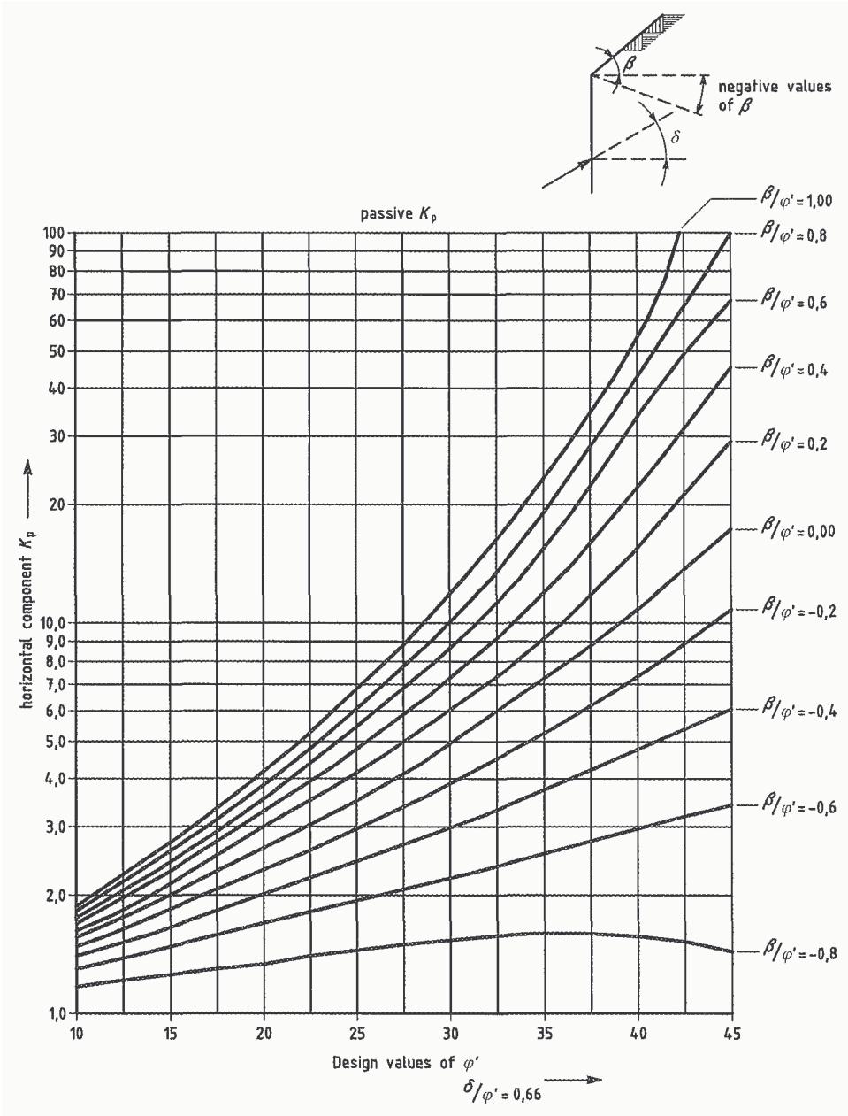
Figure C.2.3 — Coefficients K_p of passive earth pressure: with inclined retained surface ( \delta/\varphi' = 0,66 )
