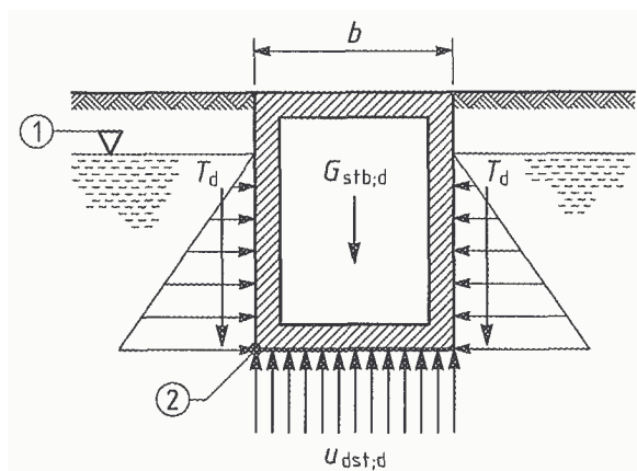
a) Uplift of a buried hollow structure
