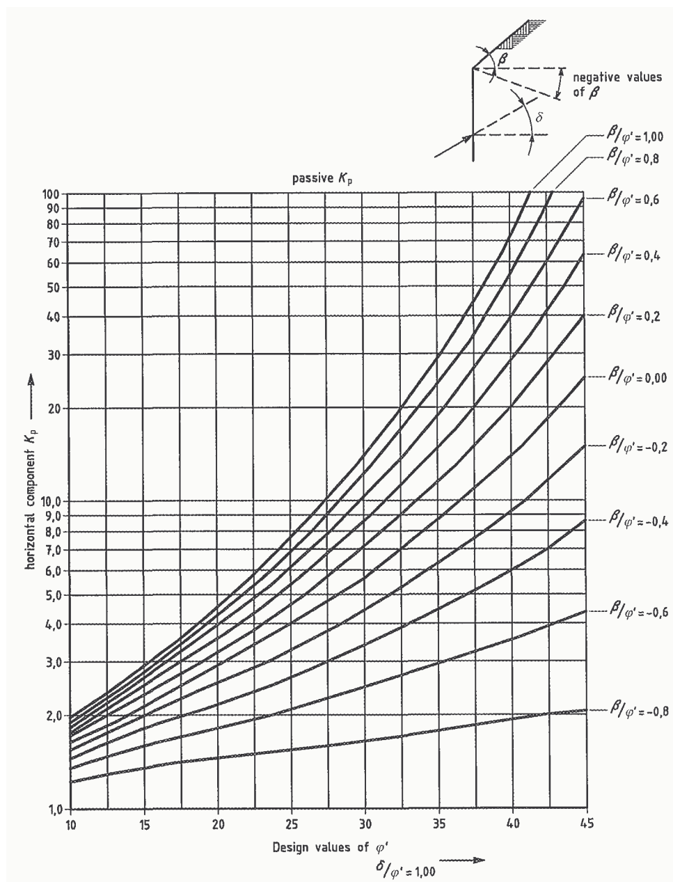
Figure C.2.4 — Coefficients K_p of passive earth pressure: with inclined retained surface ( \delta/\varphi' = 1 )
