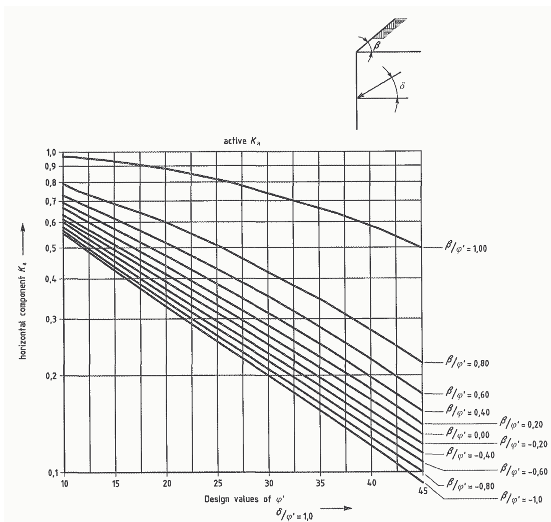
Figure C.1.4 — Coefficients K_a of active earth pressure: with inclined retained surface ( \delta/\varphi' = 1 )
