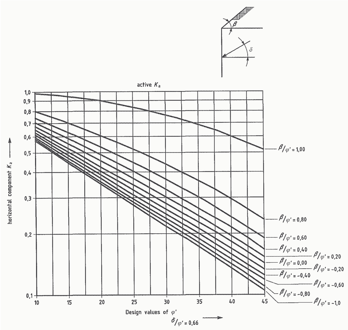
Figure C.1.3 — Coefficients K_a of active earth pressure: with inclined retained surface ( \delta/\varphi' = 0,66 )
