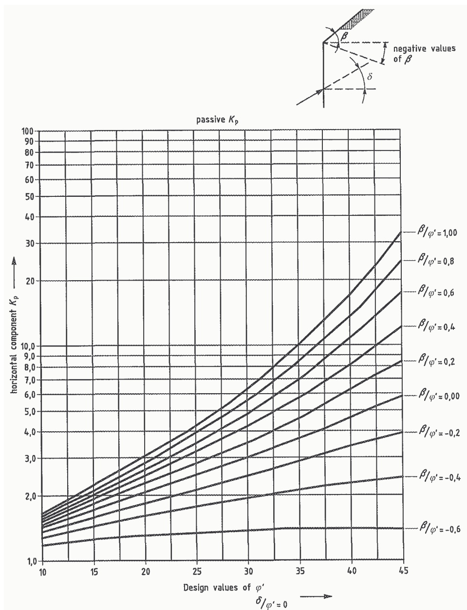
Figure C.2.2 — Coefficients K_p of passive earth pressure: with inclined retained surface ( \delta/\varphi' = 0 and \delta = 0 )
