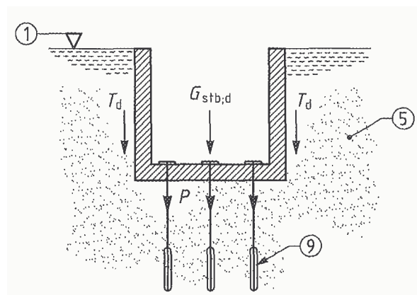
e) Structure anchored to resist uplift
