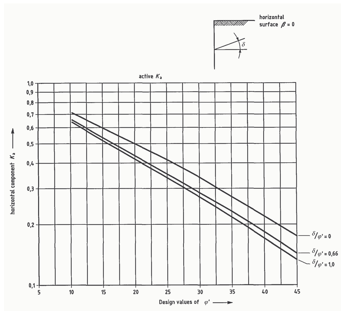
Figure C.1.1 — Coefficients K_a of active earth pressure: with horizontal retained surface ( \beta = 0 )
