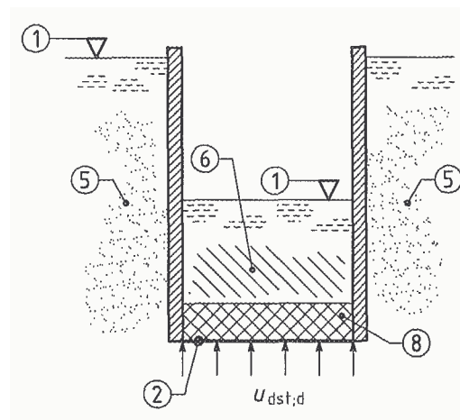
d) Execution of a slab below water level
